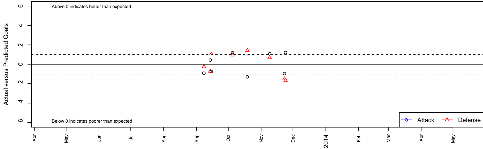
Bay Oaks SC United B96 Dots are actual minus expected GF (blue circles) and GA (red triangles). Blue line is smoothed change in attack strength. Red is smoothed change in defense strength.
